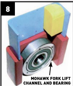
▲ FORK LIFT CHANNEL & bearing (bottom) vs. competitive columns & plastic slider (top)
