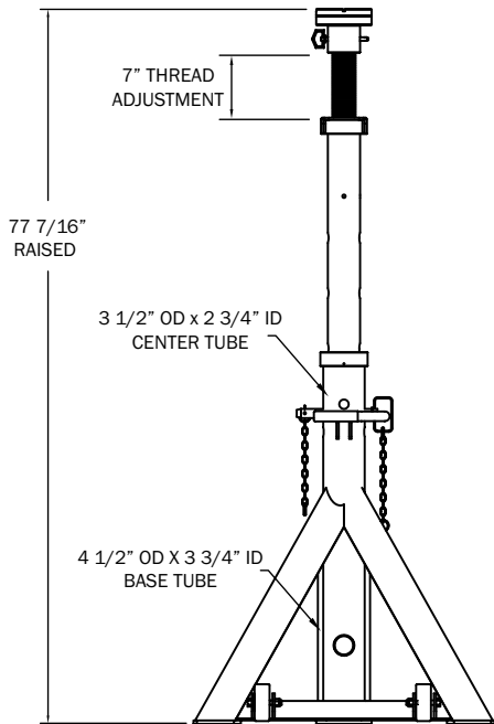
Model: JS-4775-20 20,000 lb
