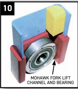
10 ▲ FORK LIFT CHANNEL & bearing (bottom) vs. competitive columns & plastic slider (top)
