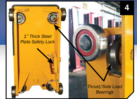
▲ LiftPoint's welded steel carriages roll on eight double sealed, self-lubricating, steel ball bearing rollers, and incorporates a thrust load bearing design to dissipate the thrust from heavy counterbalanced forklifts.
