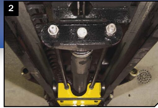
▲ Heavy duty column construction with direct drive cylinders, direct drive lifting rods and stainless steel hydraulic lines are built for decades of low-maintenance operation.
